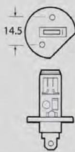
P14.5s
